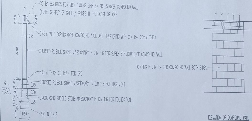
CROSS SECTION ON A-B
